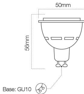
Base: GU10
