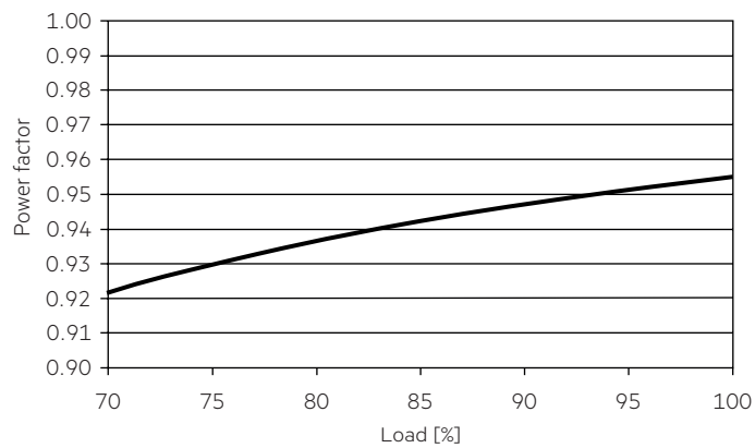
4.4.2 Power factor vs load
