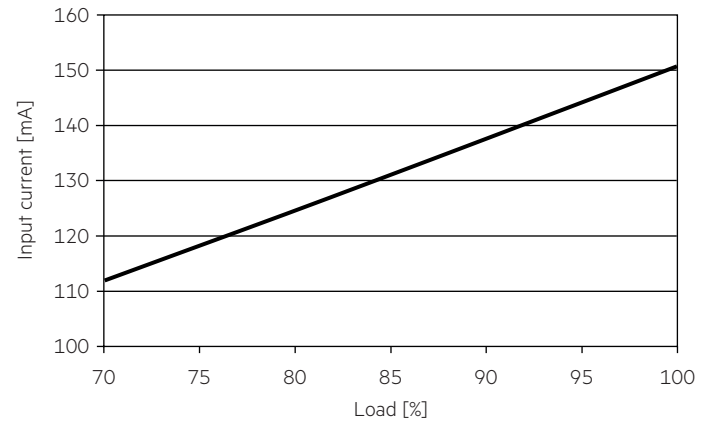
4.4.4 Input current vs load
