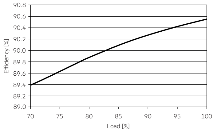
4.4.1 Efficiency vs load
