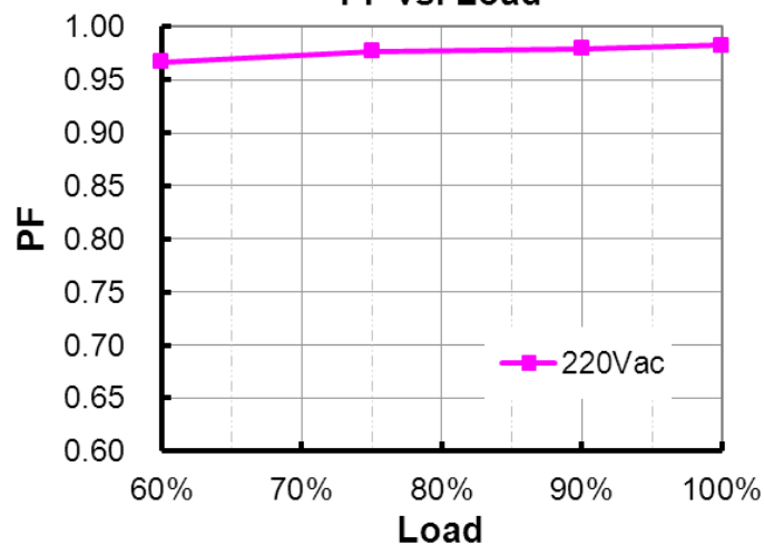
PF vs. Load
