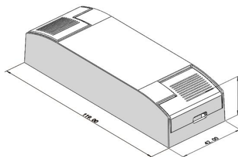
Gyrometer (L x W x H): 119 x 42 x 25mm
