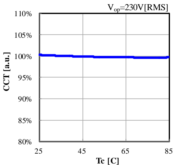
Case Temperature vs. CCT
